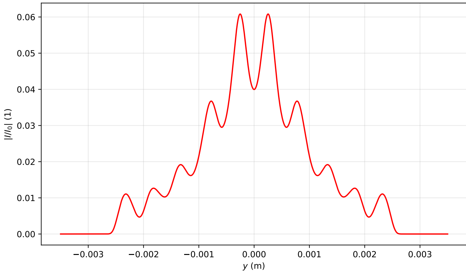
Intensity profile I(x=0, y, z=3.662)/I_0 , P_{in}=2.0P_{cr} , artificial time
